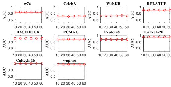
Fig. 6. Sensitivity Test Results w.r.t. \alpha on Ten Data Sets.
