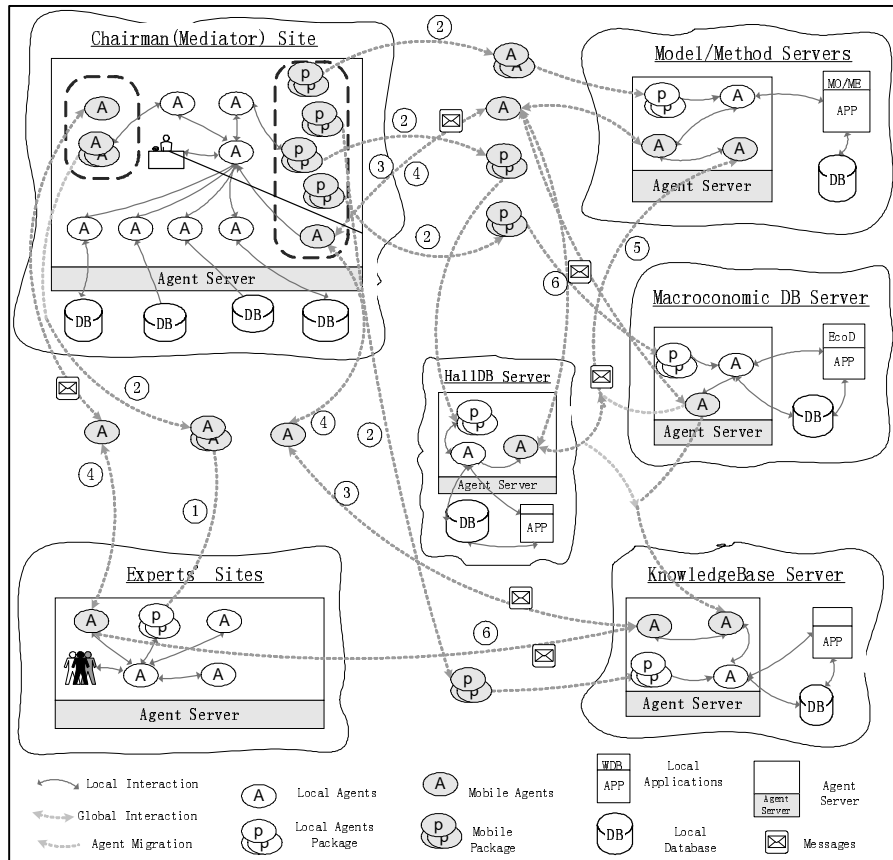
Fig.2 System structure of multi-agent-based macroeconomic decision support system
