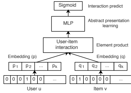
Figure 2: DeepCF: learning implicit user-item couplings.
