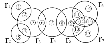
Figure 4: Coverage of R on T' .
