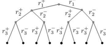
Figure 3: Enumeration process.
